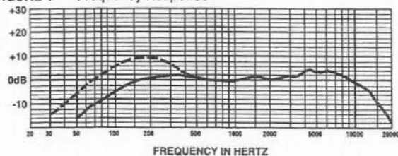
FIGURE 1 — Frequency Response
